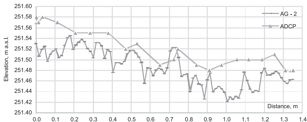
Fig. 4. Longitudinal riverbed profile, section of the Skawa River, sample S1-4
