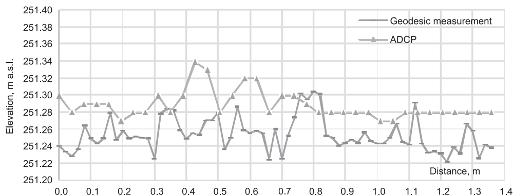
Fig. 5. Longitudinal riverbed profile, section of the Skawa River, sample S3-3
