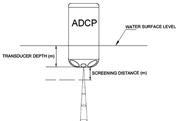
Fig. 3. Scheme of the parameters defining the operation of the ADCP probe
