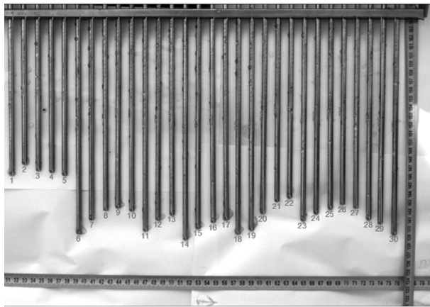
Fig. 1. Distribution of rods of the AG-2 profilometer, Skawa River at kilometre 19+293
