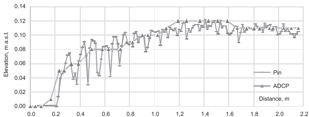
Fig. 6. Longitudinal profile, section of the Skawa River, sample L2-10
